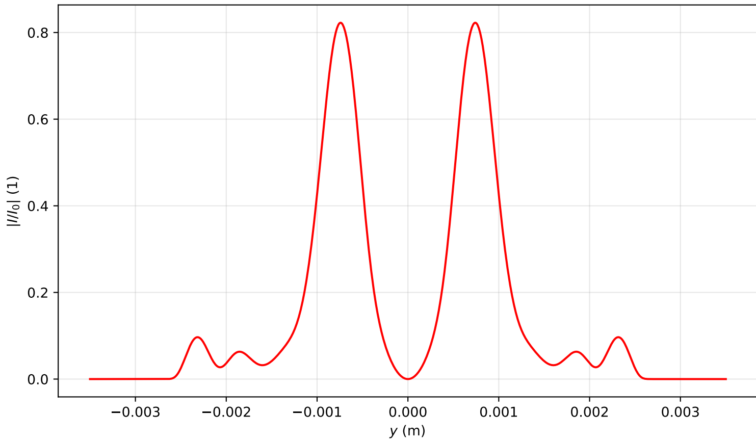
Intensity profile I(x=0, y, z=3.582)/I_0 , P_{in}=5.0P_{cr} , artificial time
